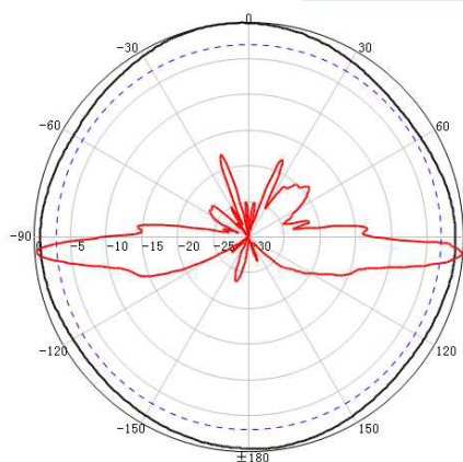
H-Pol @ 5550MHz
