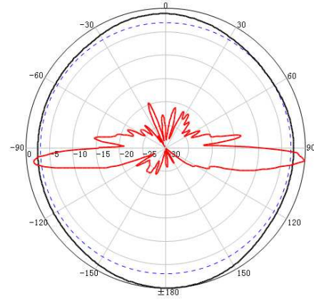
V-Pol @ 5550MHz
