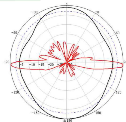
V-Pol @ 2450MHz
