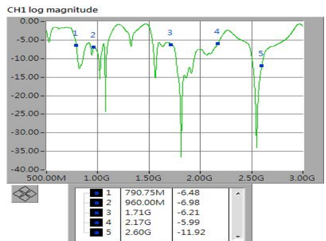
S11
